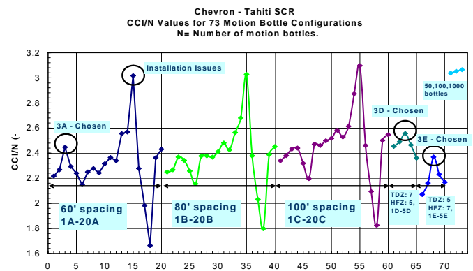
Figure 5 – Configuration Clarity Indices for 73 Motion Bottle Arrangements
