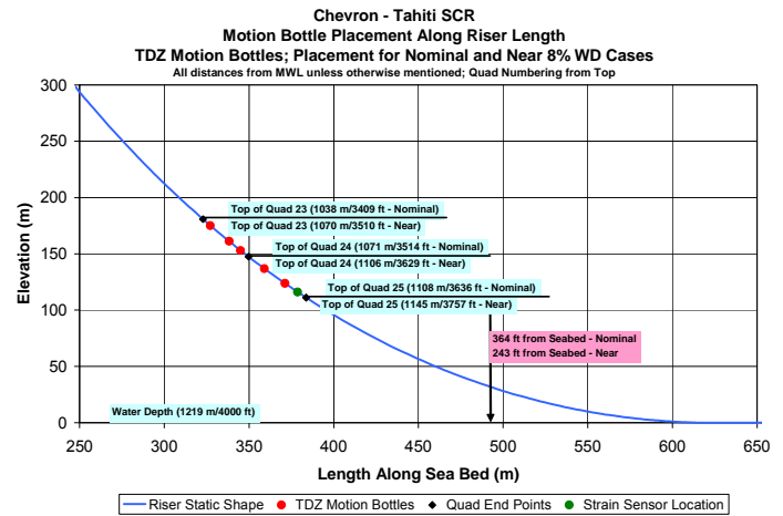
Figure 10 – Optimized (Final) Motion Bottle Location
