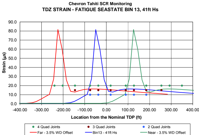
Figure 9 – 100 yr TDZ Strain vs Monitoring Locations Combined Motion and Strain Sensor Placement Strategy
