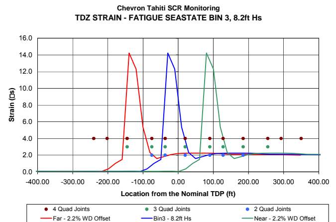
Figure 7 – 1 yr TDZ Strain vs Monitoring Locations
