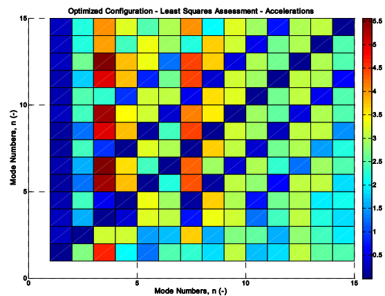
Figure 11 – Modal Clarity Matrix, Optimized for Motion Bottle Placement
