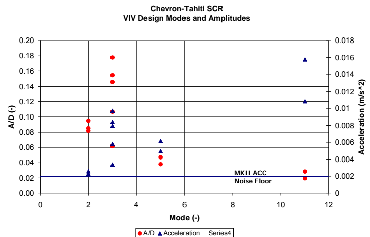
Figure 14 - VIV Response Analysis of Tahiti SCR and Comparison of Acceleration Amplitudes with Motion Sensor Accuracy
