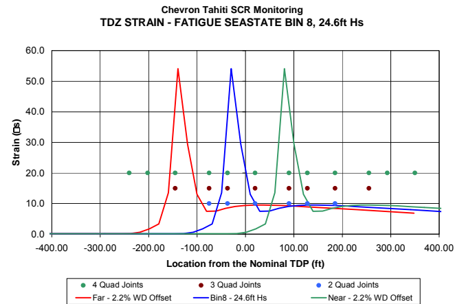
Figure 8 – 10 yr TDZ Strain vs Monitoring Locations
