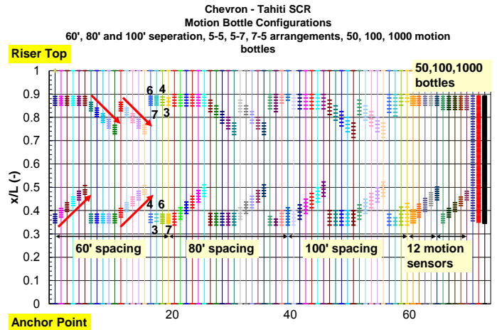
Figure 4 – Motion Sensor Arrangement Assessed
