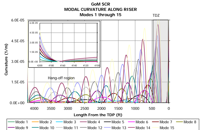
Figure 18 –SCR Modal Curvature
