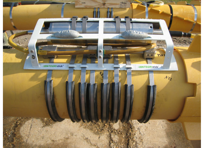
Figure 3 – INTEGRISTICK Dynamic Curvature Sensor Installed on SCR Joint
