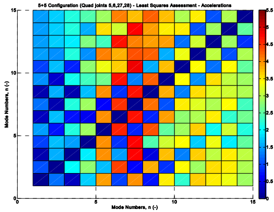
Figure 12 – Modal Clarity Matrix, Motion Sensors in Quads Adjacent to Strain Sensors
