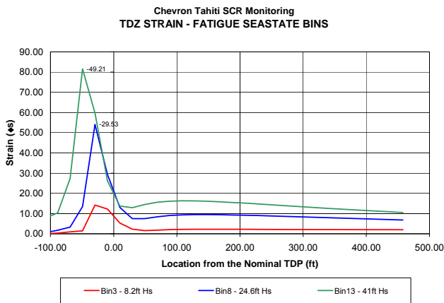
Figure 6 – Touch Down Region Strain Distribution
