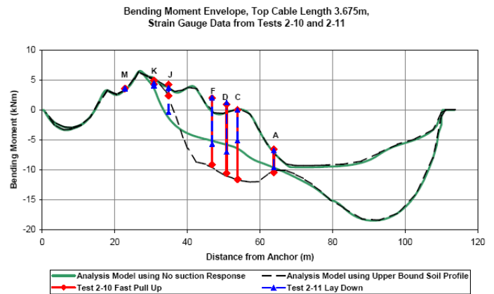
Figure 20 –Soil Suction Model Calibration, STRIDE JIP
