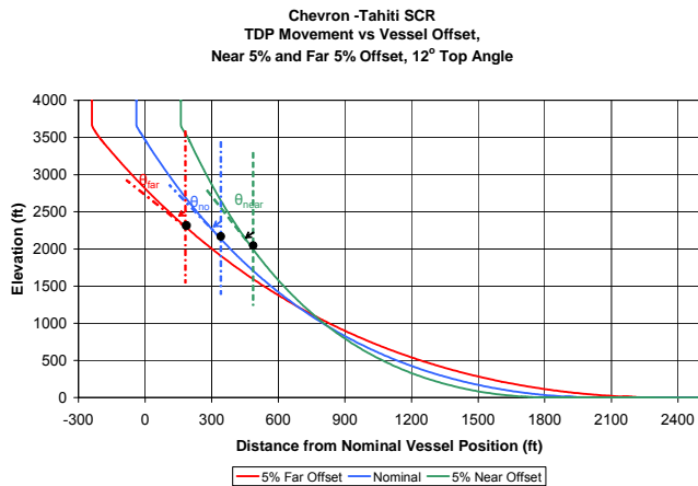
Figure 19 –SCR Catenary Angle Calculation
