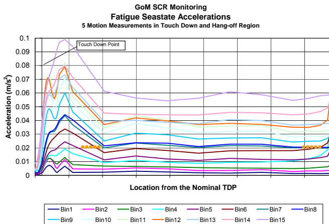
Figure 15 – Riser Accelerations for a Typical GoM SCR
