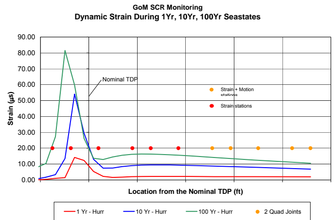
Figure 16 – Extreme Storm Riser Strains for a Typical GoM SCR
