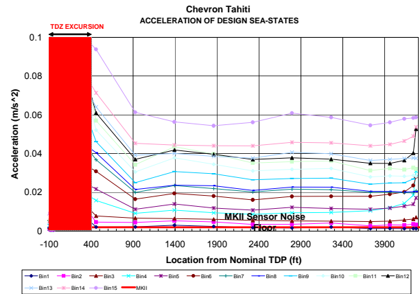
Figure 13 – Wave/Vessel Motion Induced Riser Accelerations with Motion Sensor Accuracy
