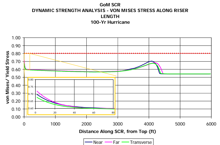
Figure 17 – Dynamic Stress along the Riser
