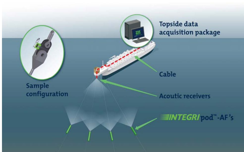
Figure 7 – moorASSURE™ Monitoring System Schematic Description
