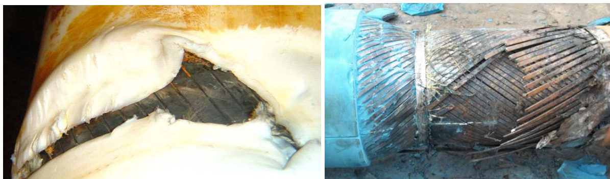
Figure 5 – Left: External Sheath Damage Caused by Bend Stiffener Contact at the I-Tube (2).
