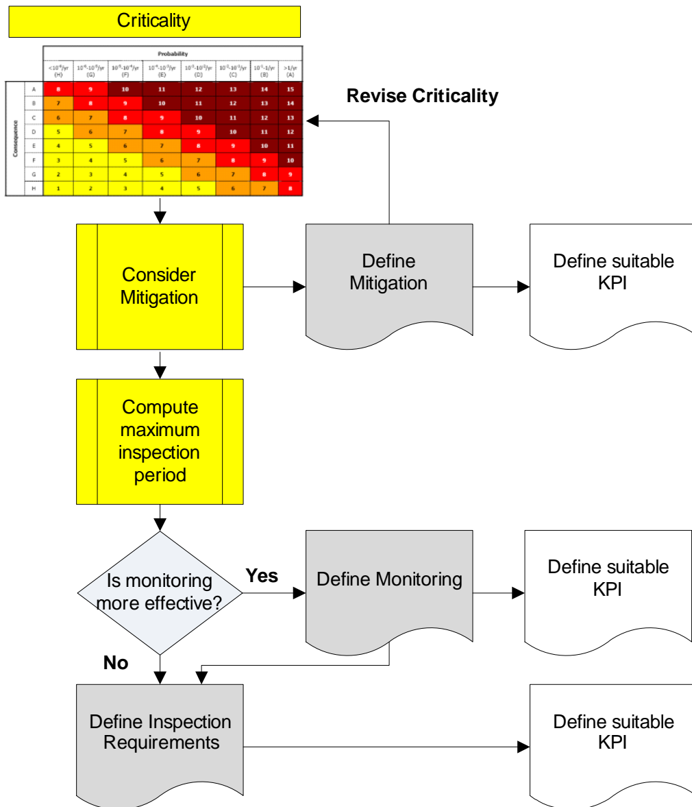
Figure 1 - Integrity Assessment Process
