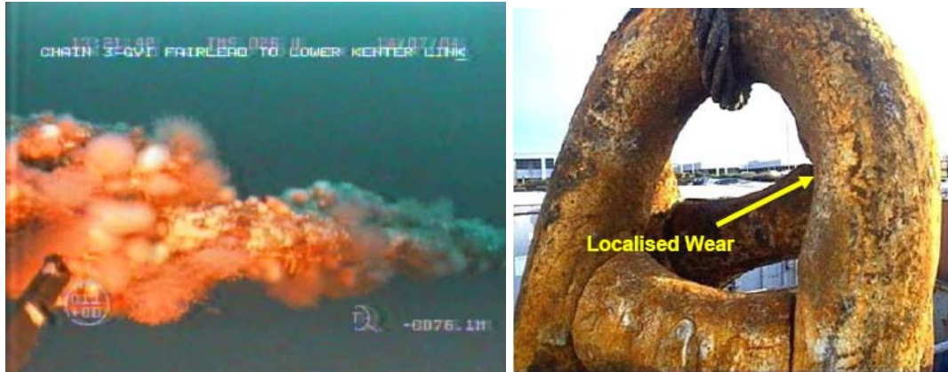
Figure 3 – Left: Excessive Marine on a Long Term Deployed Chain (3).
