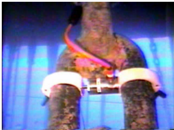
Figure 12 – Left: INTEGRicuff – Dynamic Chain Monitoring Device, installed in P-35 FPSO, offshore Brazil.
