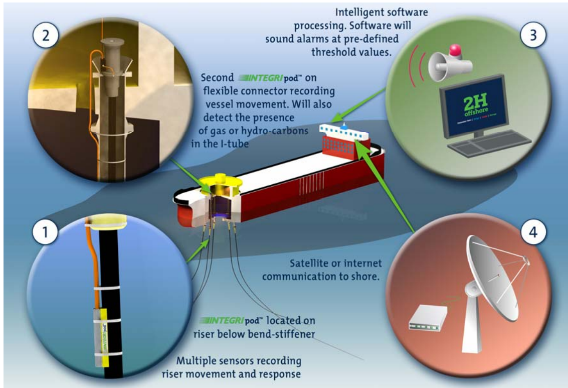
Figure 8 – flexASSURE™ Monitoring System Components Overview
