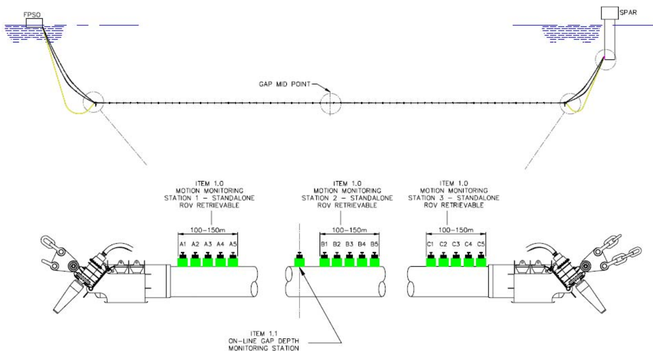
Figure 3 – Bundled Mid-Water Flowline Monitoring System
