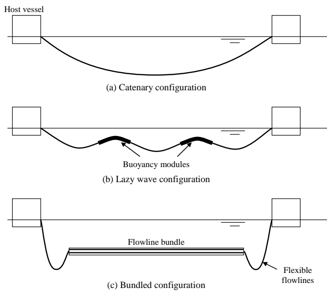
Figure 1 – Mid-Water Flowline Configurations
